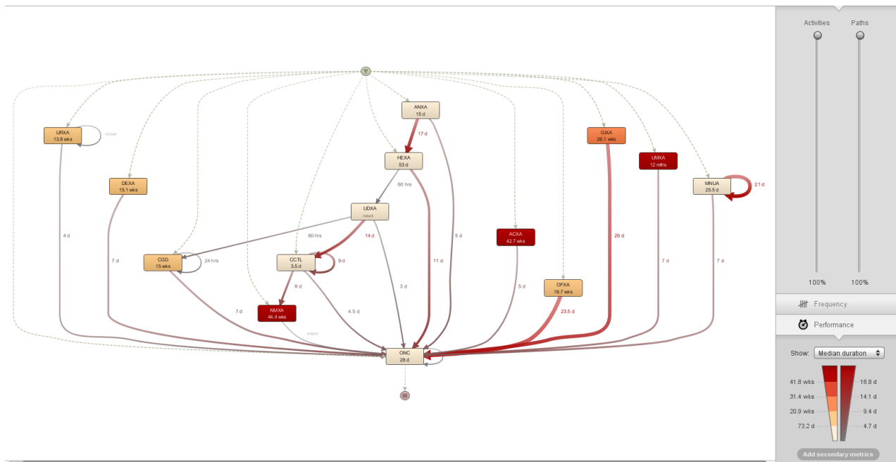
Figure 7: Process map in Disco after filtering events
